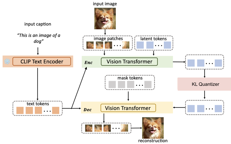
Figure 6: TextTok-VAE: Text-aware 1D Tokenizer Architecture.
