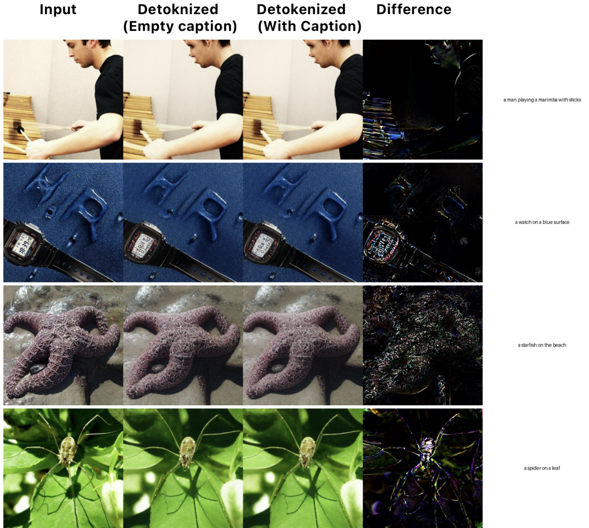
Figure 12: Effect of text guidance on image tokenization. The “Detokenized” column displays reconstructed images with and without text guidance. The “Difference” columns highlight the texture details missed in the reconstruction when no caption is provided, emphasizing the improvements text guidance brings to capturing finer image details.
