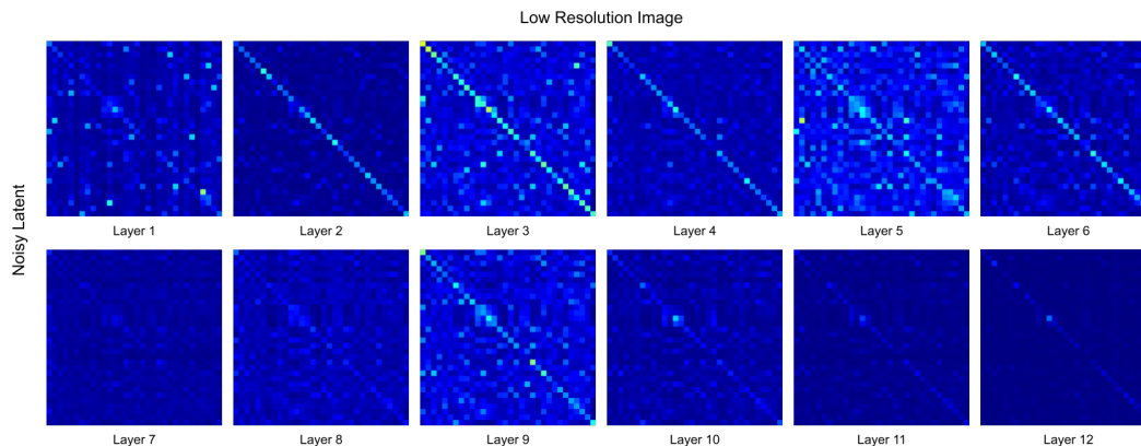
Figure 16: Self-Attention Maps for TaTiTok
