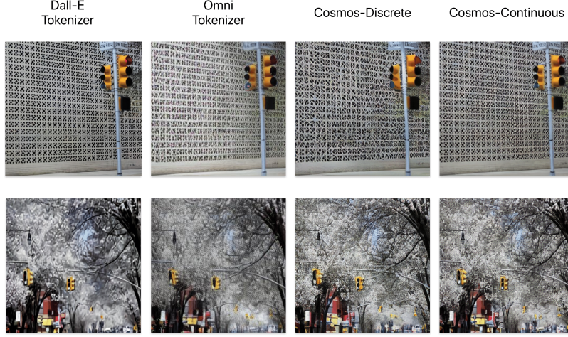
Figure 5: Tokenizer Baseline Qualitative Results
