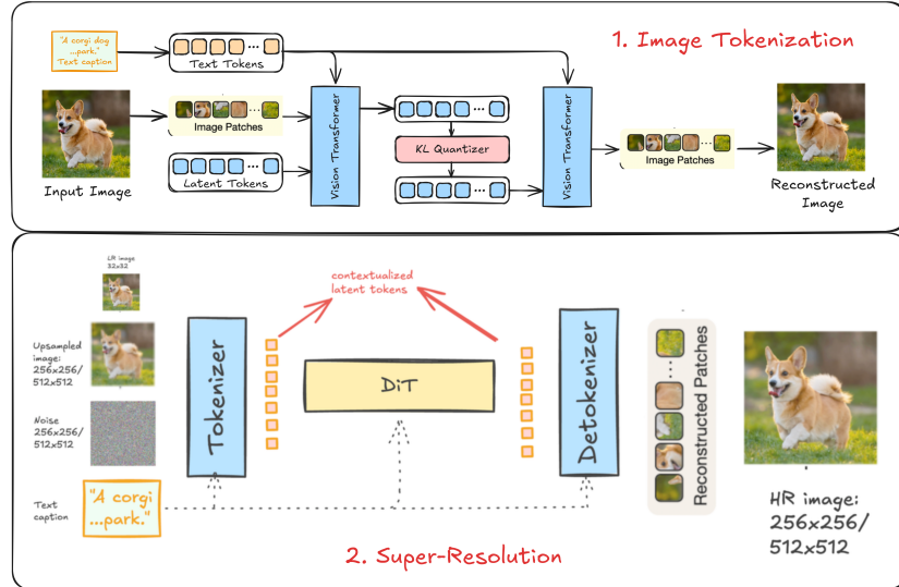
Figure 1: Overview of Proposed Image Tokenization and Super-Resolution Architectures
