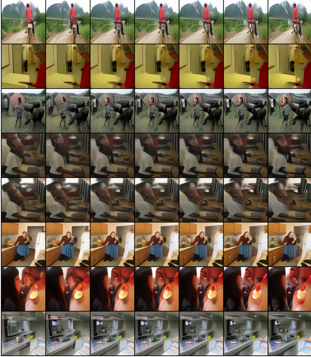
Figure 14: Evaluating the impact of guidance scale on super-resolution. Column 1 is the output of a simple tokenization-detokenization process which we treat as the ground truth. The columns after show the output of the SR model at guidance scales [0, 2, 4, 6, 8, 10] .
