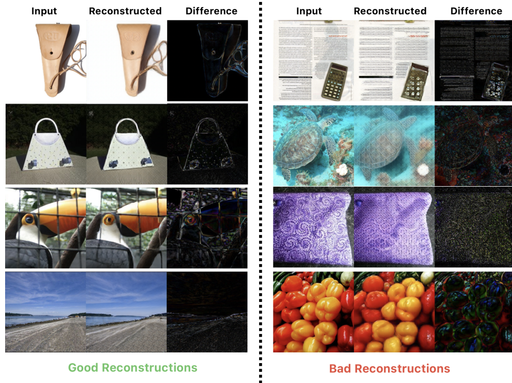
Figure 11: Reconstruction results from TexTok-VAE. This figure showcases both successful reconstructions and cases where the tokenizer struggles to encode the input into the compact 1D latent space of 32 tokens. Difference images are provided to highlight discrepancies between the reconstructed and original images, illustrating areas where the model’s tokenization fails to capture fine details.
