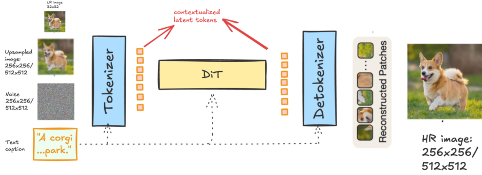
Figure 7: Overall achitecture of our approach
